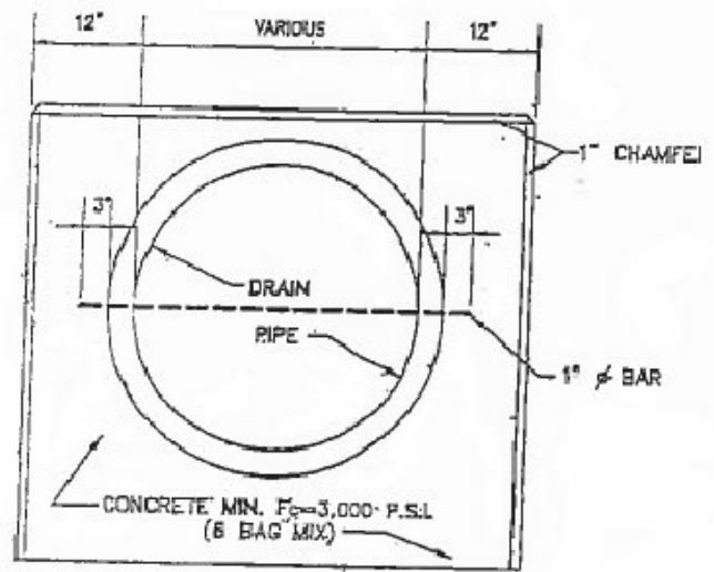
FRONT ELEVATION
