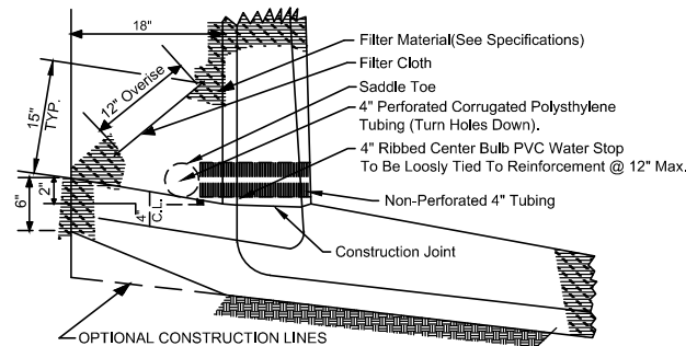
WATER STOP DETAIL (TYPICAL SECTION)
