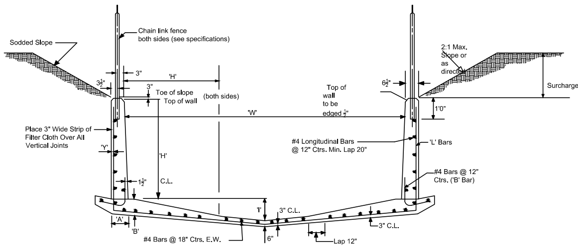
TYPICAL SECTION
