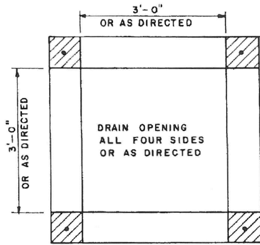
PLAN SECTION A-A
