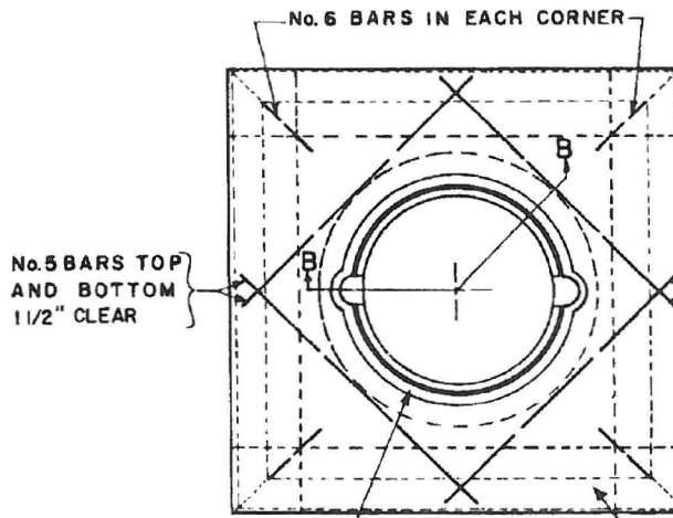
TOP PLAN
