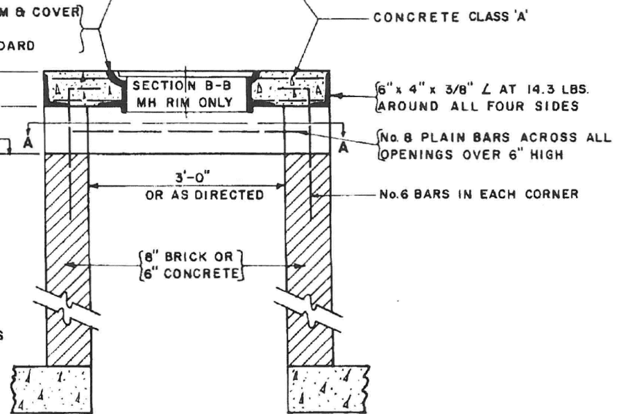
SECTION OVER CONCRETE BOX CULVERT
