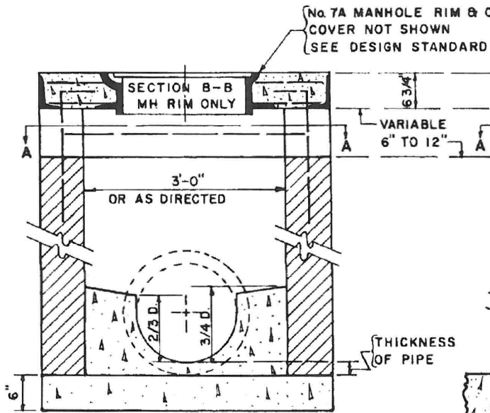
SECTION OVER PIPE
