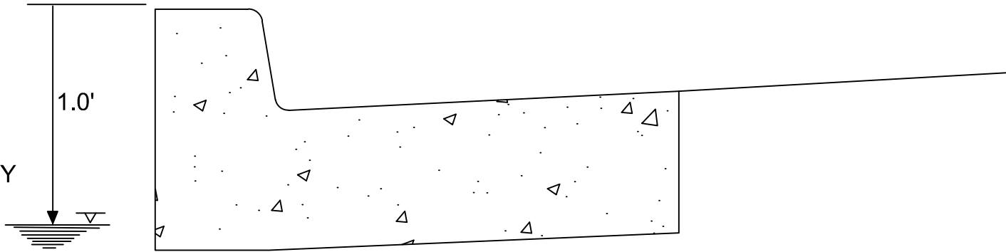
TYPICAL CURB & GUTTER
