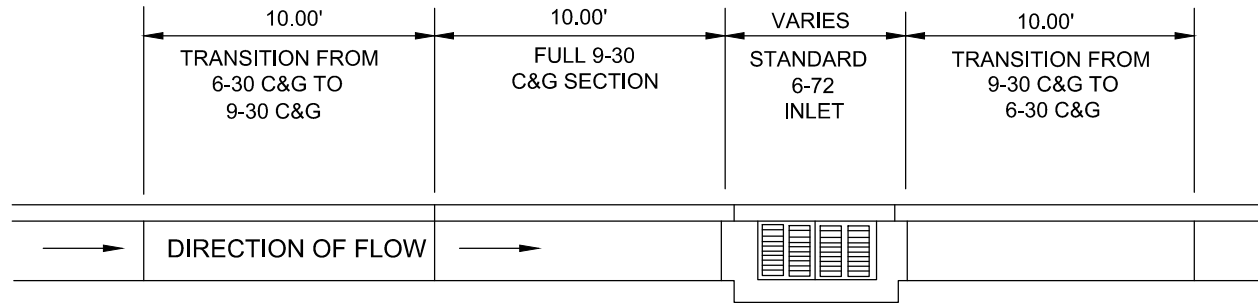
9-30 CURB AND GUTTER
