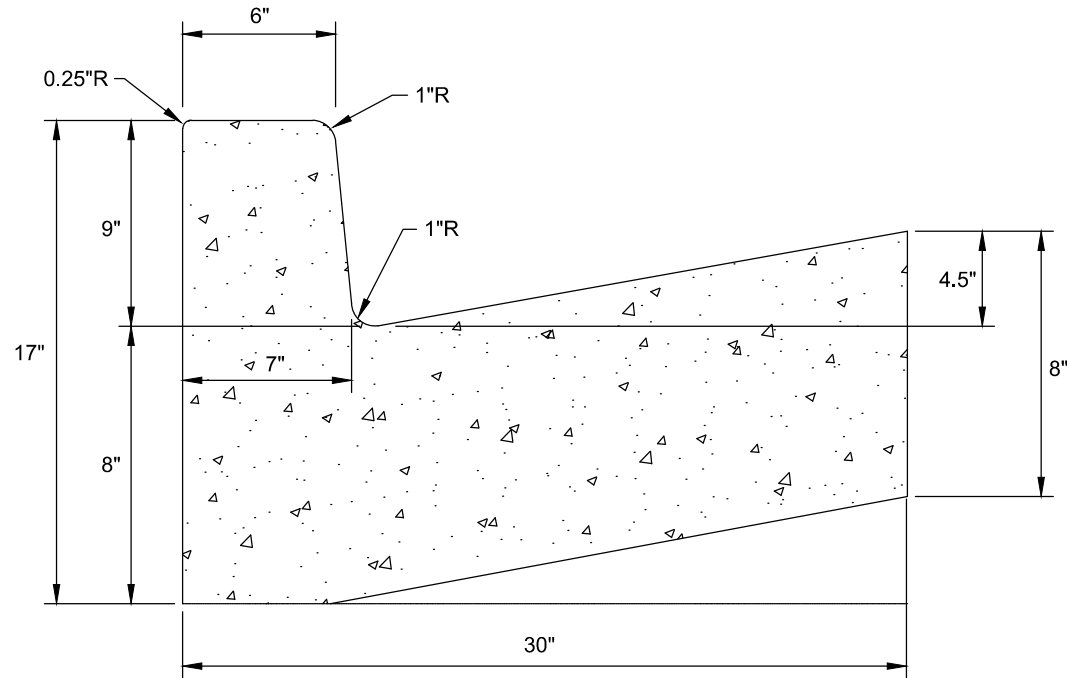
9-30 CURB AND GUTTER
