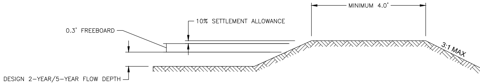
DIVERSION BERM
