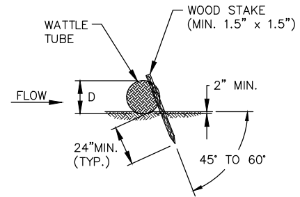
STAKING DETAIL
