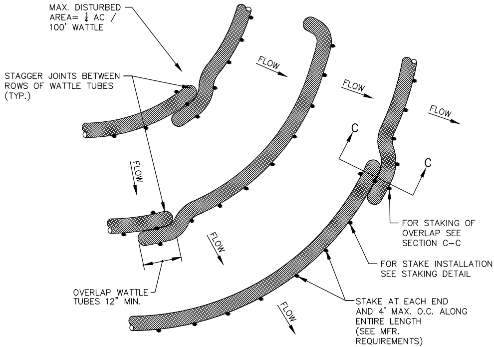
PLAN VIEW FOR SLOPE APPLICATION
