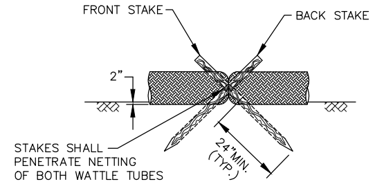
JOINT STAKING DETAIL
