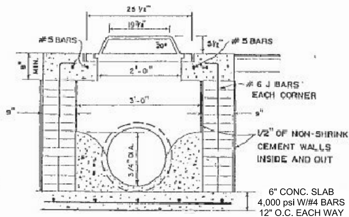
CROSS SECTION
