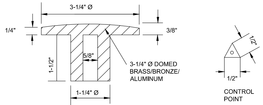
A-A STANDARD SUBDIVISION CORNER/WITNESS DISK CROSS-SECTION
